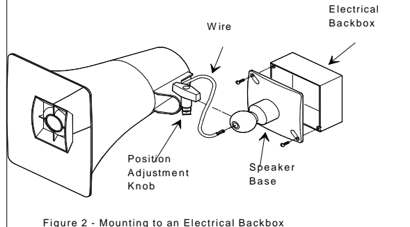
Figure 2 - Mounting to an Electrical Backbox
