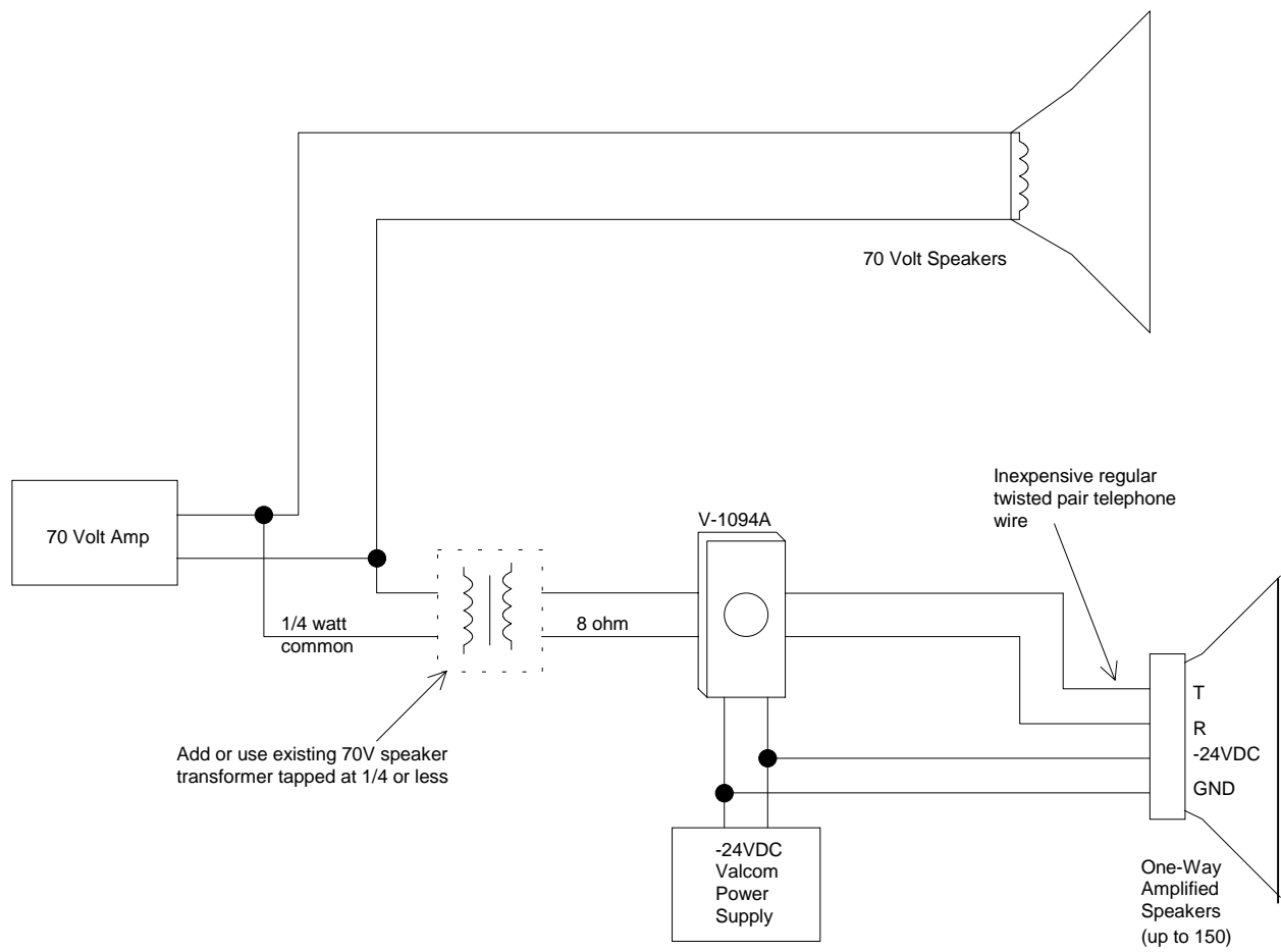
FIGURE 2 - CONNECTIONS TO 25 OR 70 VOLT PAGING SYSTEM
