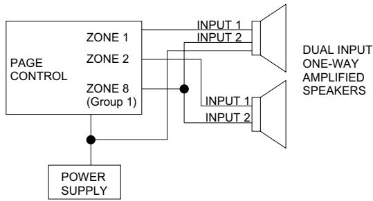
FIGURE 3 - GROUP CALL BLOCK DIAGRAM
