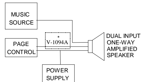
FIGURE 2 - PAGE SYSTEM BLOCK DIAGRAM
